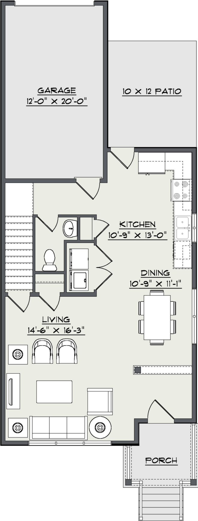
First Floor
