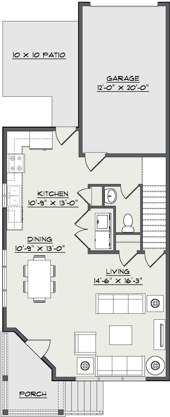
First Floor
