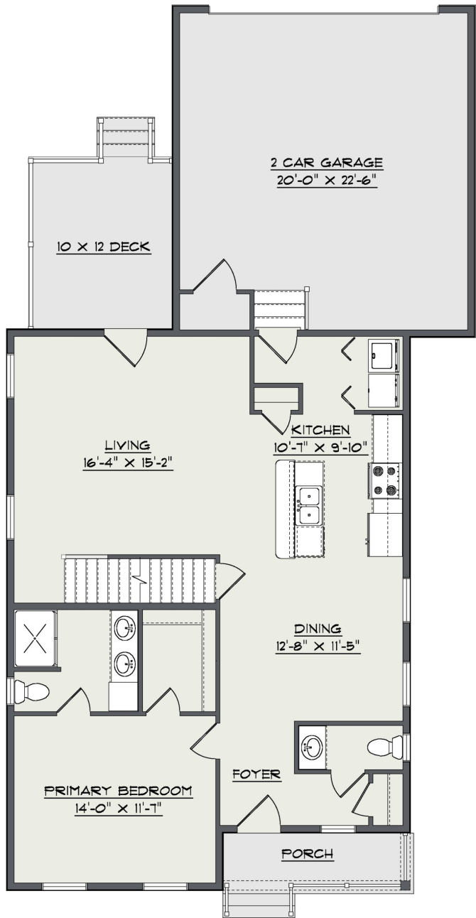
First Floor
