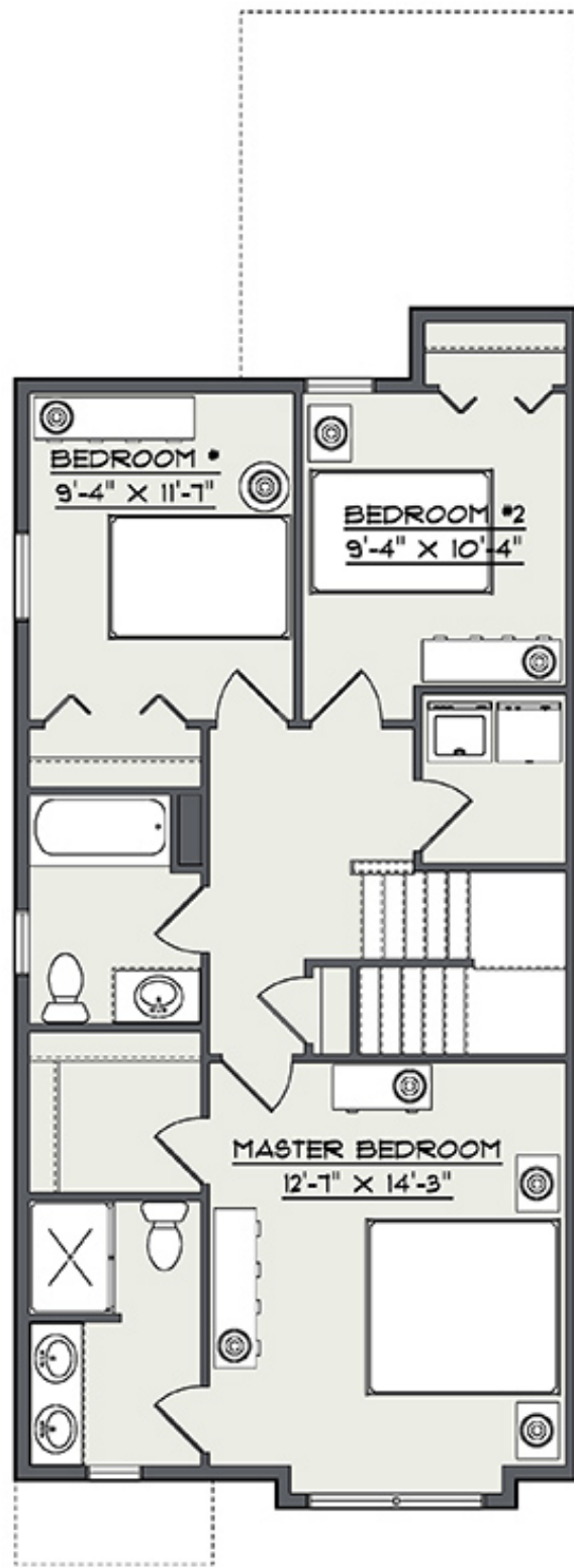
Second Floor
