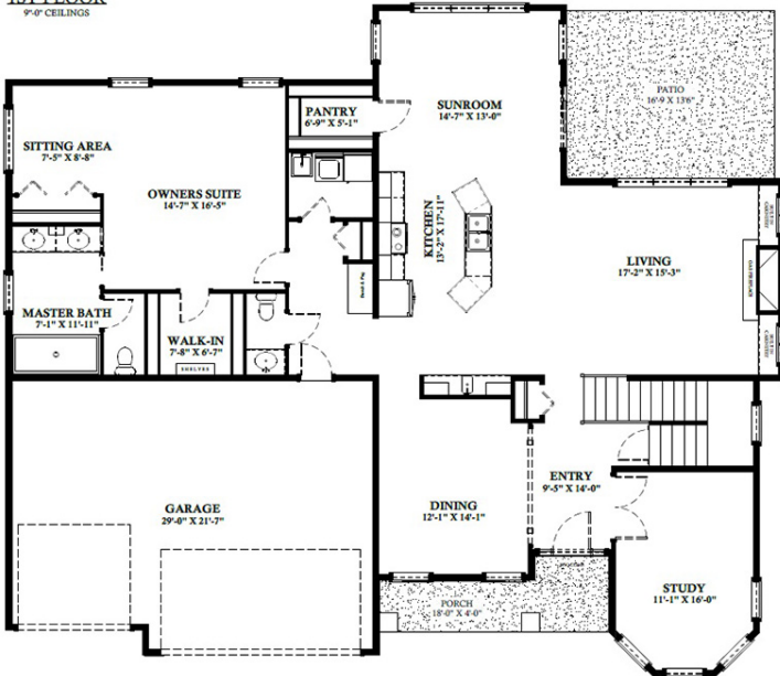
1ST FLOOR 9'-6" CEILINGS
