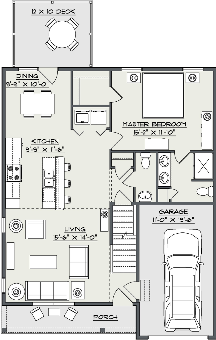
First Floor
