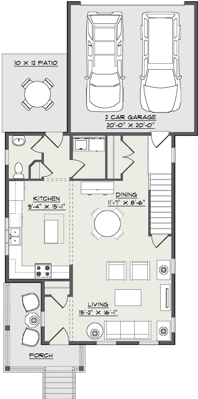
1st Floor plans
