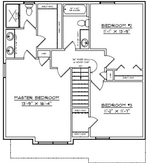
SECOND FLOOR PLAN SCALE: 3/8" = 1'-0"
